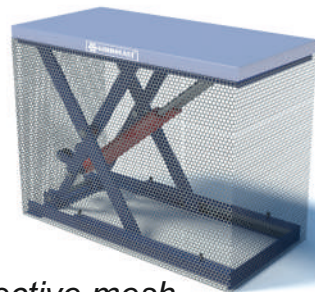
Protective mesh
